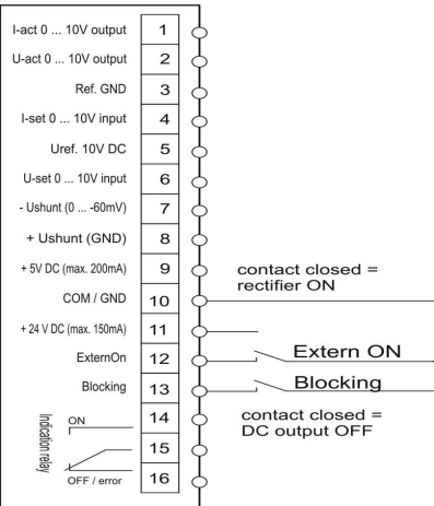
X5-Service terminal
