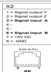
BUS output
